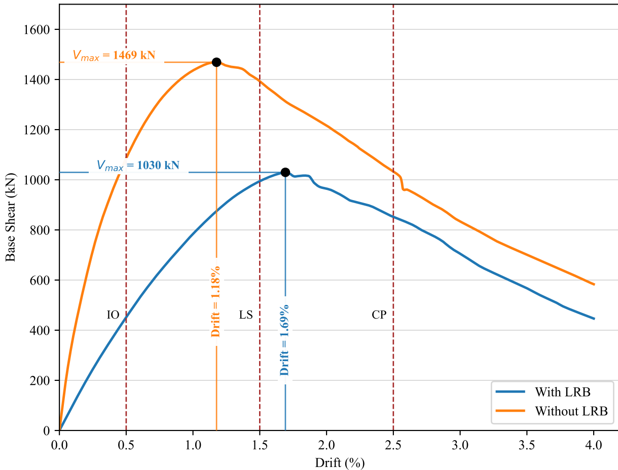
Pushover Curves for 750kL Tank
